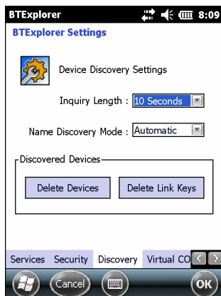
Figure 4-33 BTE Explorer Settings - Discovery
