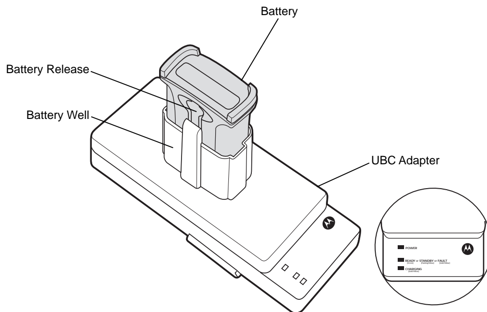
Figure 5-15 UBC Adapter
