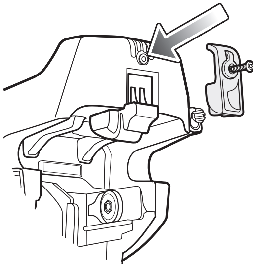
Figure 5-23 Locking Mechanism
